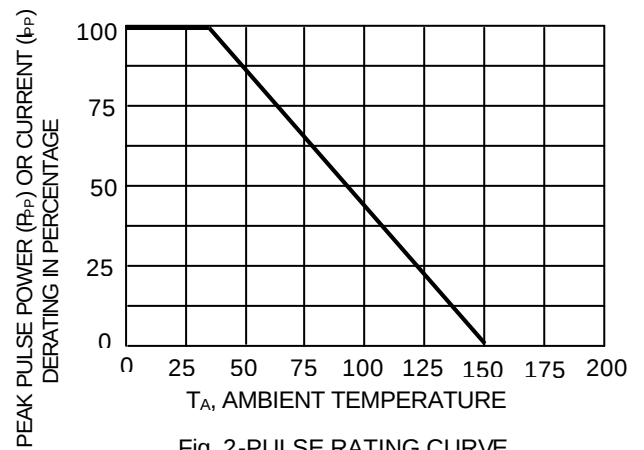
Fig. 2-PULSE RATING CURVE
